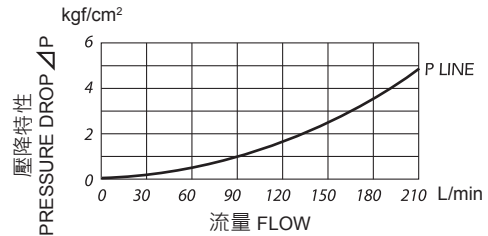
閥軸全開時壓力降特性 PRESSURE DROP AT SPOOL FULLY OPENED
