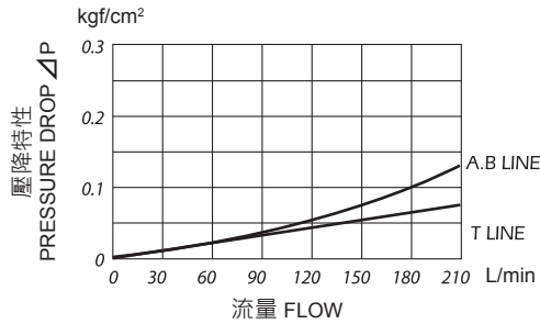
壓力降特性 PRESSURE DROP
