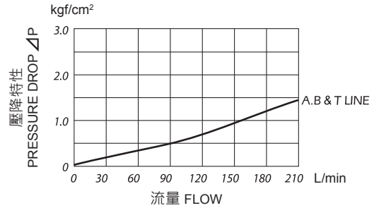
壓力降特性 PRESSURE DROP
